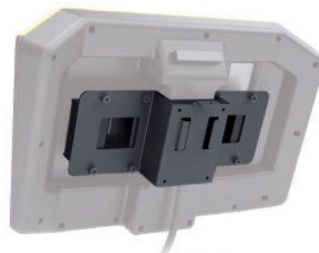
Removable holder is attached from the back
